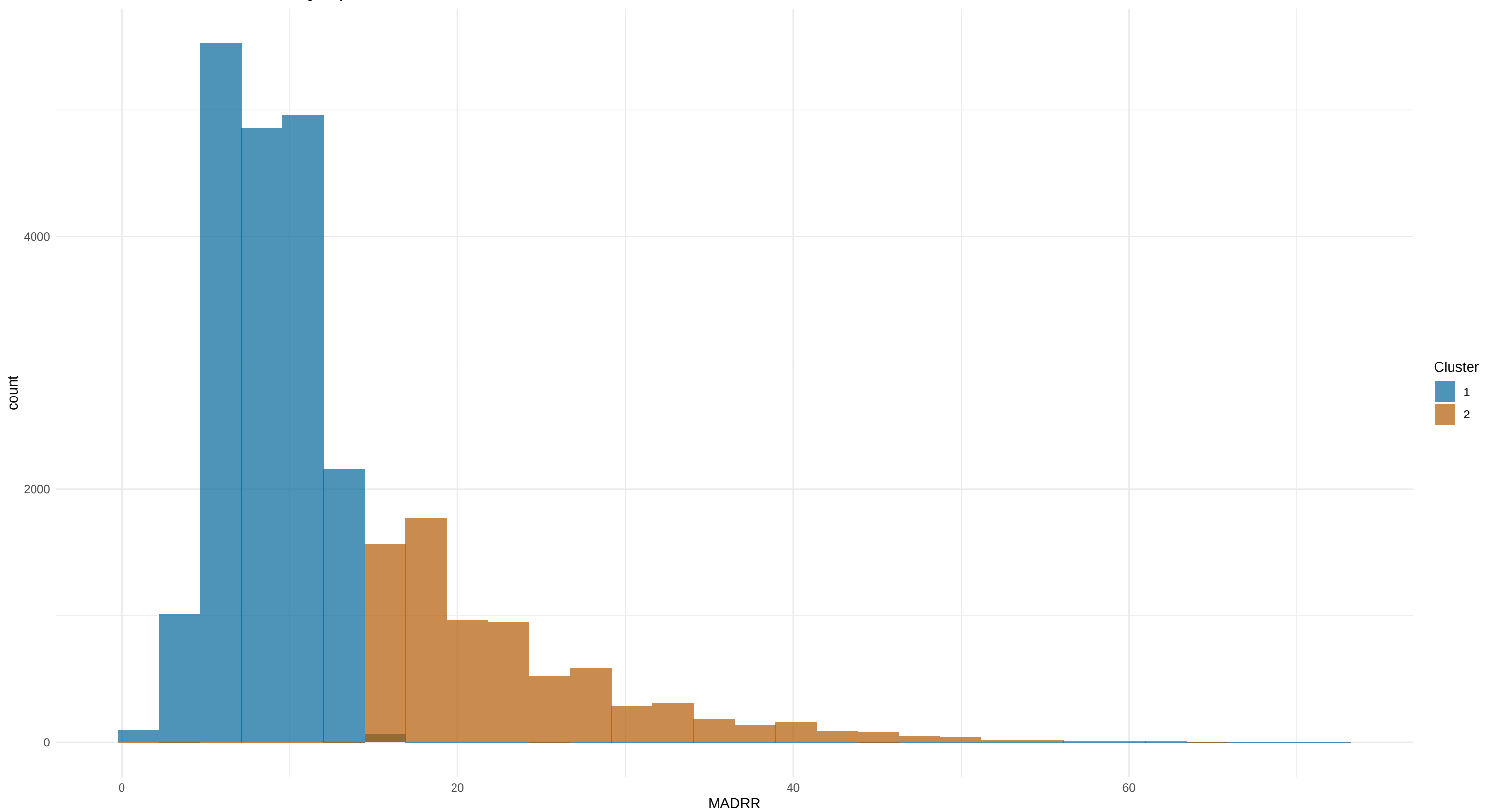
MADRR clustered into automatic groups
